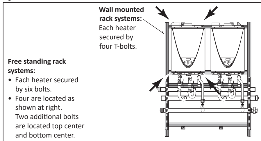
Figure 7: T-bolt indicator (wall mounted racks only).
