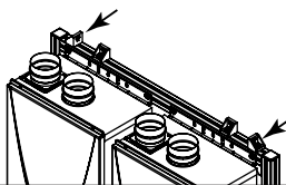
Figure 1: Lifting Brackets
