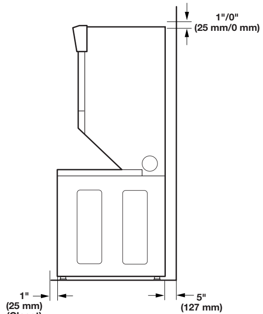
Front/Back/Top clearances
