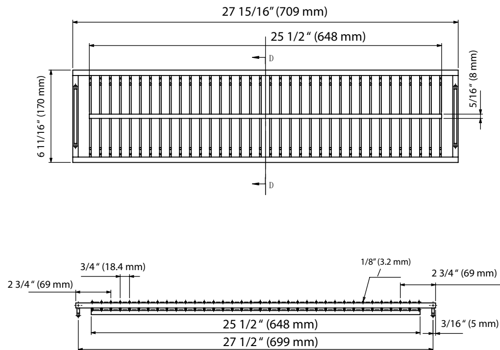
Warming Rack
