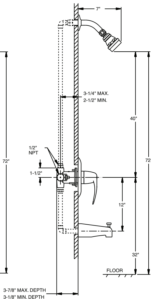
Tub/Shower Installation
