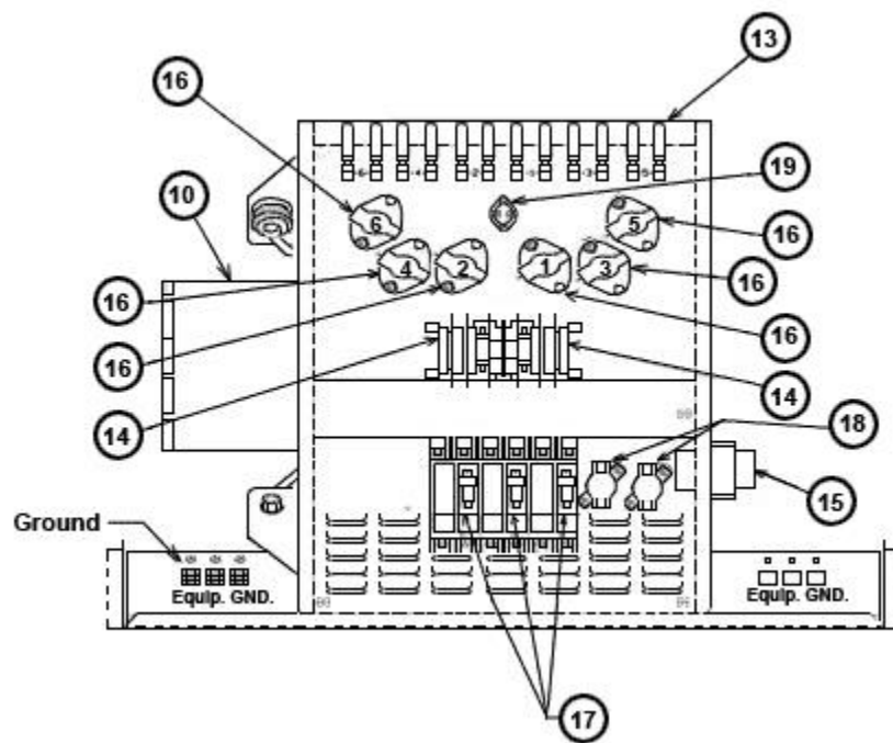
Electrical Assembly
