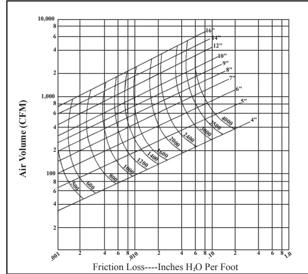
Straight lines -- Nominal Duct ID Curved lines -- Velocity in fpm
