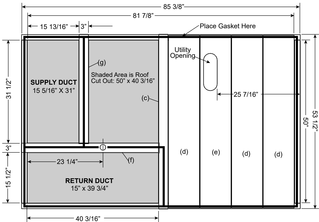
Figure 5 - Top View
