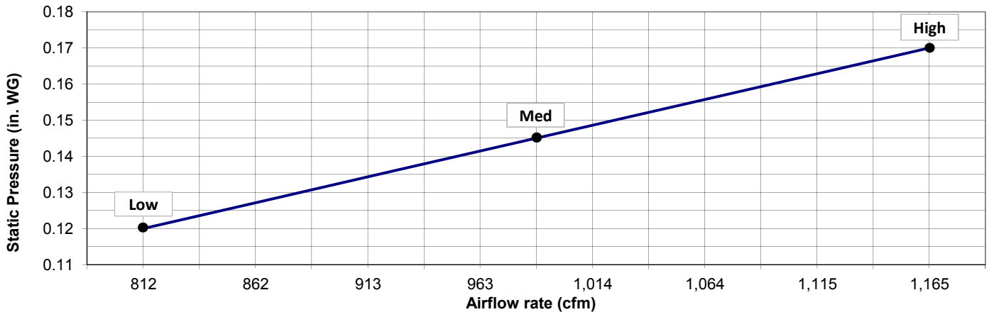
PEFY-P36-NMAU-E2 with Filter Box FBM2-4
