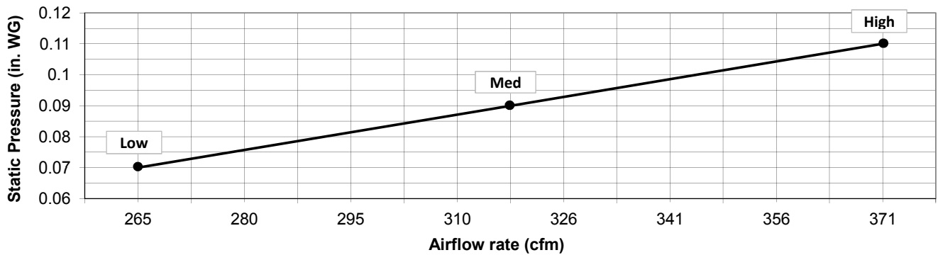
PEFY-P12-NMAU-E2 with Filter Box FBM2-1
