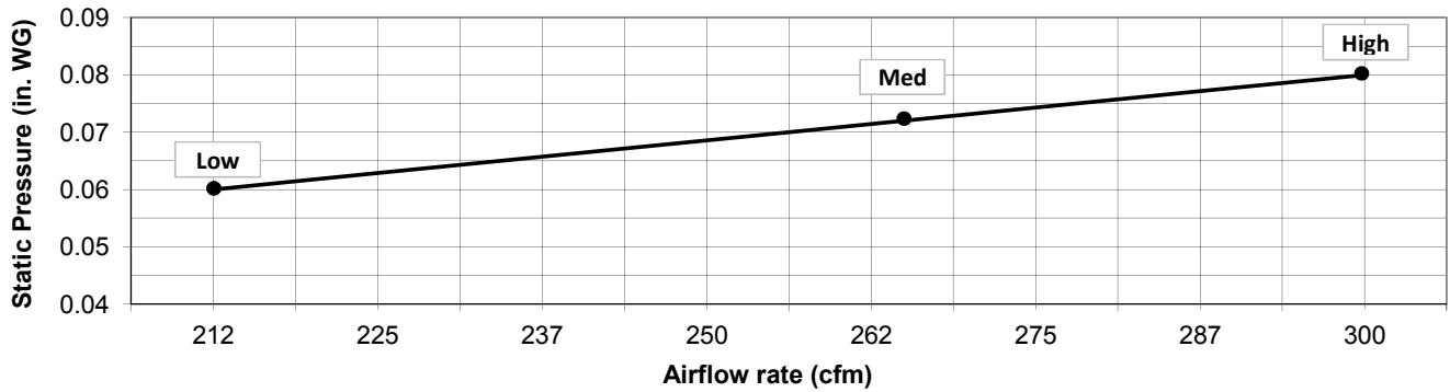
PEFY-P06, P08-NMAU-E2 with Filter Box FBM2-1
