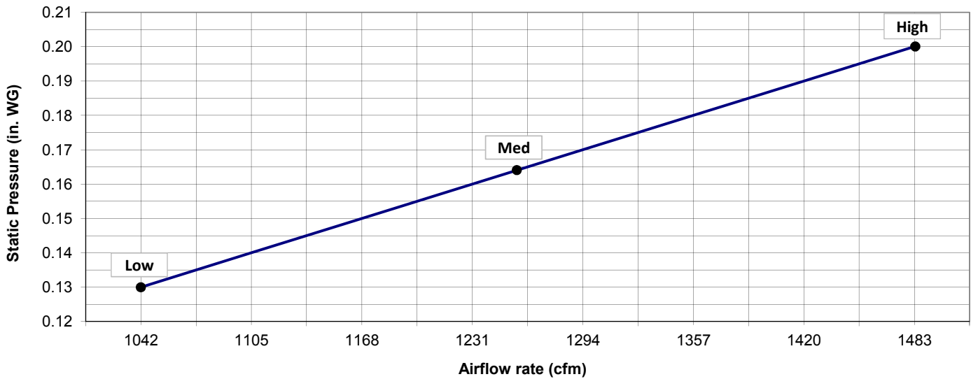
PEFY-P54-NMAU-E2 with Filter Box FBM2-5
