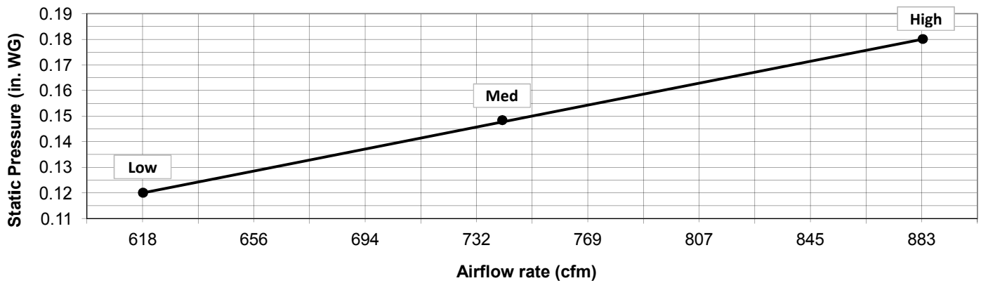
PEFY- P24, P27, P30-NMAU-E2 with Filter Box FBM2-3
