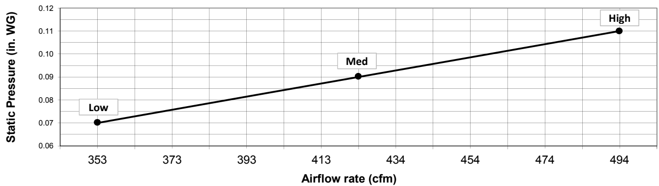
PEFY-P15-NMAU-E2 with Filter Box FBM2-2
