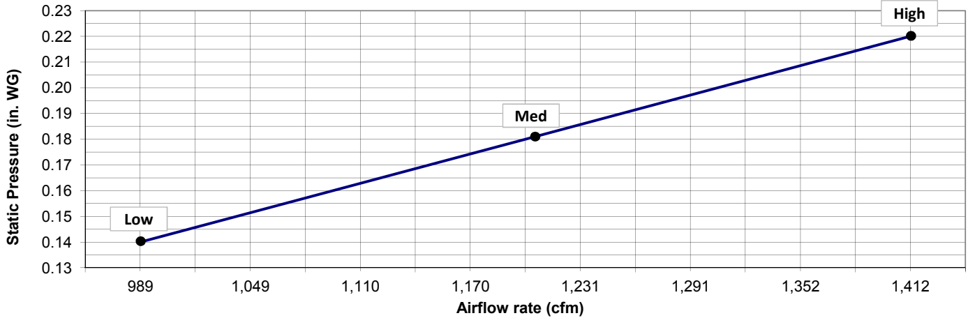
PEFY-P48-NMAU-E2 with Filter Box FBM2-4
