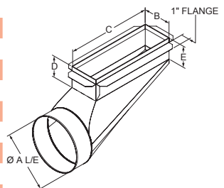
End Boot with 1" Flange
