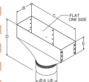
Universal Boot
