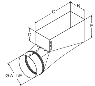
End Boot
