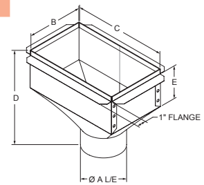
Universal Boot with 1" Flange
