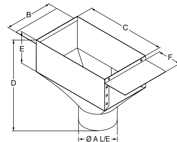
Universal Boot with 1" Flange
