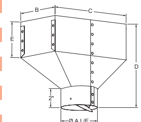
Universal Boot with Damper
