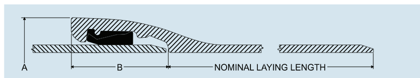
Tyton® Joint
