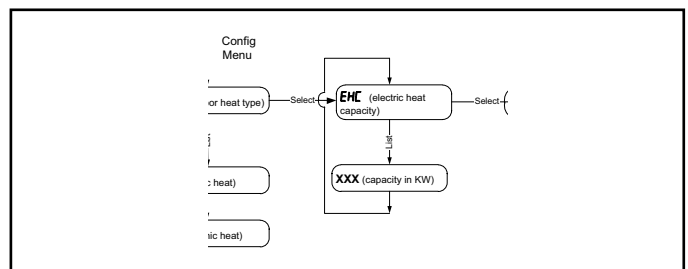
Figure 7 - Configuration Menu
