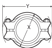
Style 907 and Style W907 Pre-Assembled (Installation-Ready Condition)
