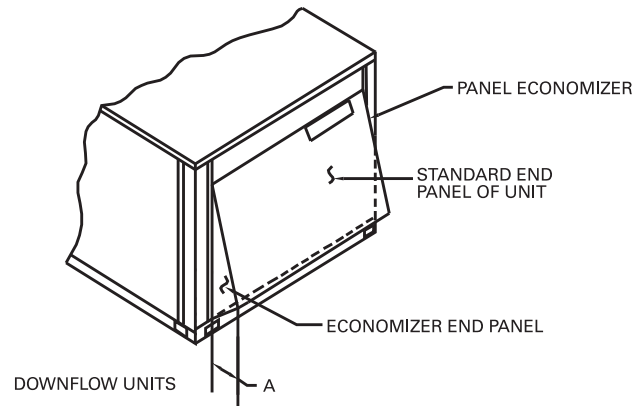
Figure 18. Economizer—downflow units
