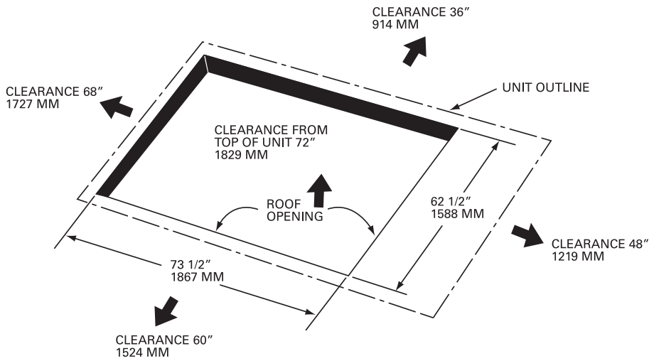
Figure 5. Cooling with optional electric heat and gas/electric models—12½ tons standard efficiency—downflow unit supply/return and unit clearance
