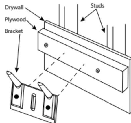
Figure 9 - Mounting for Drywall
