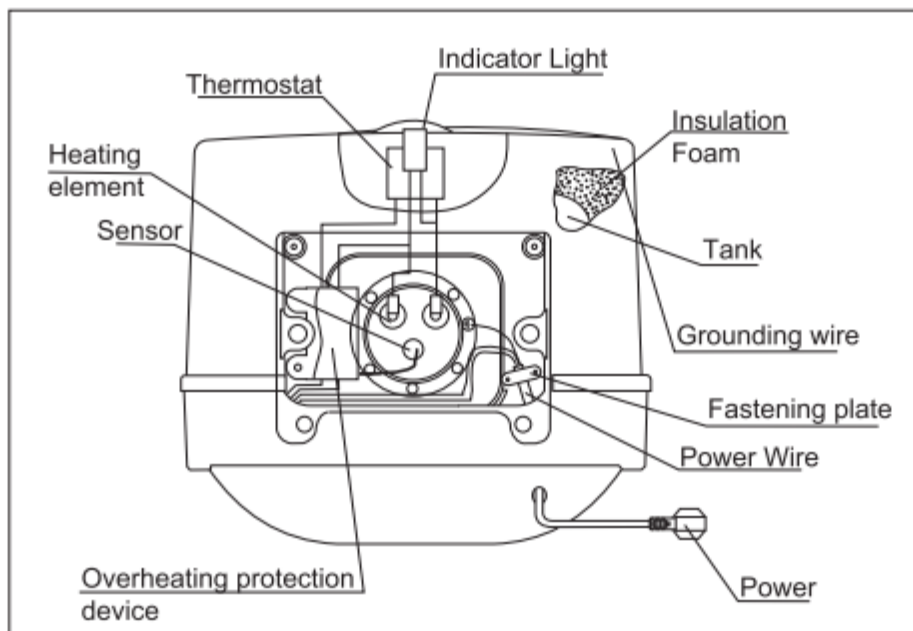
Schematic Construction
