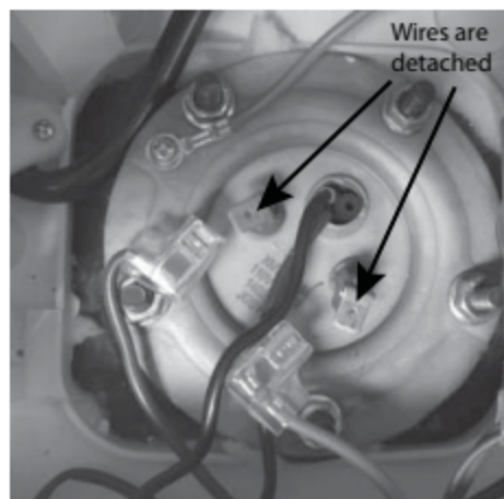
Figure 21 - Use a multimeter to check the resistance of the heating element.
