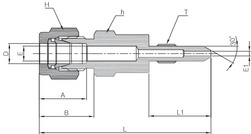
2U thread calibration fitting for Yokogawa/Rosemount DP transmitters
