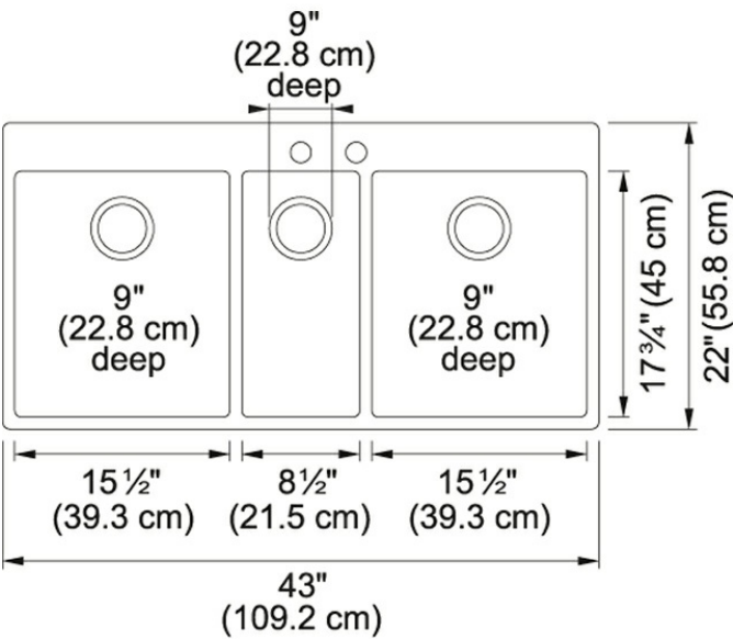
Technical Drawing
