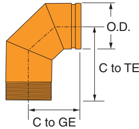
FIGURE 7055 90° ADAPTER ELBOW
