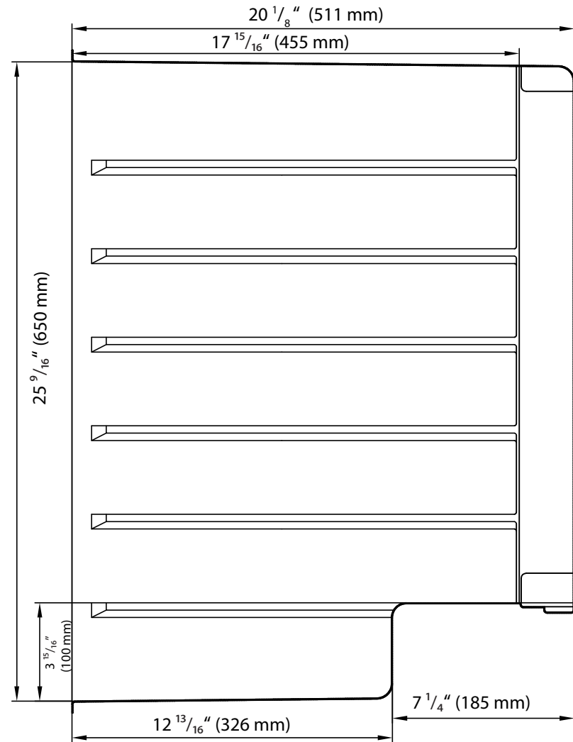
Side View
