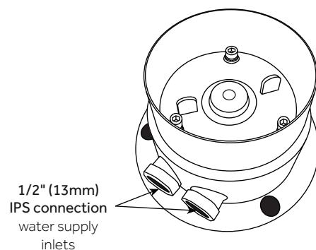
Rough-In Valve Detail
