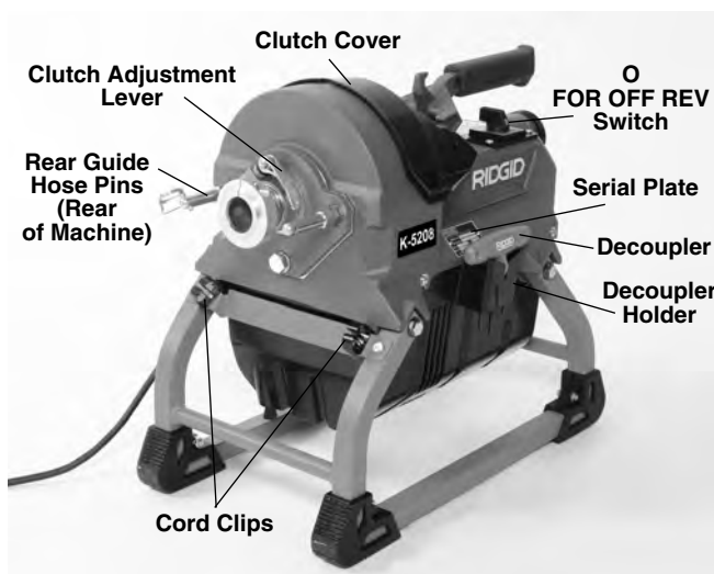
Figure 1 – K-5208 Drain Cleaning Machine
