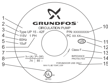
Fig. 1 Nameplate
