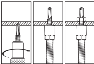
Install with appropriate sized steel socket driver. (side and variable mount direction versions not pictured)
