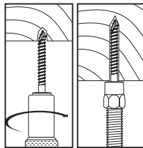
Install with appropriate sized wood socket driver. (side and variable mount direction versions not pictured)
