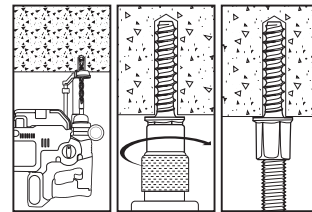
Install with appropriate sized concrete socket driver. (variable mount direction version not pictured)
