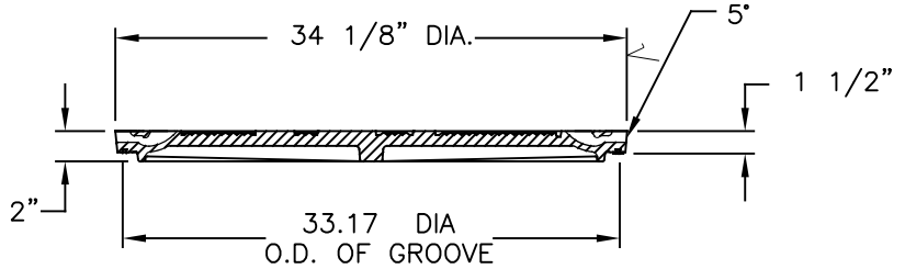
COVER SECTION
