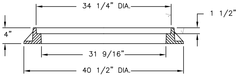
FRAME SECTION
