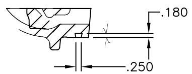
GASKET GROOVE DETAIL
