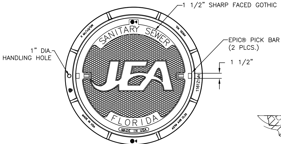
PLAN VIEW
