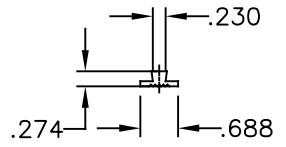
GASKET DETAIL
