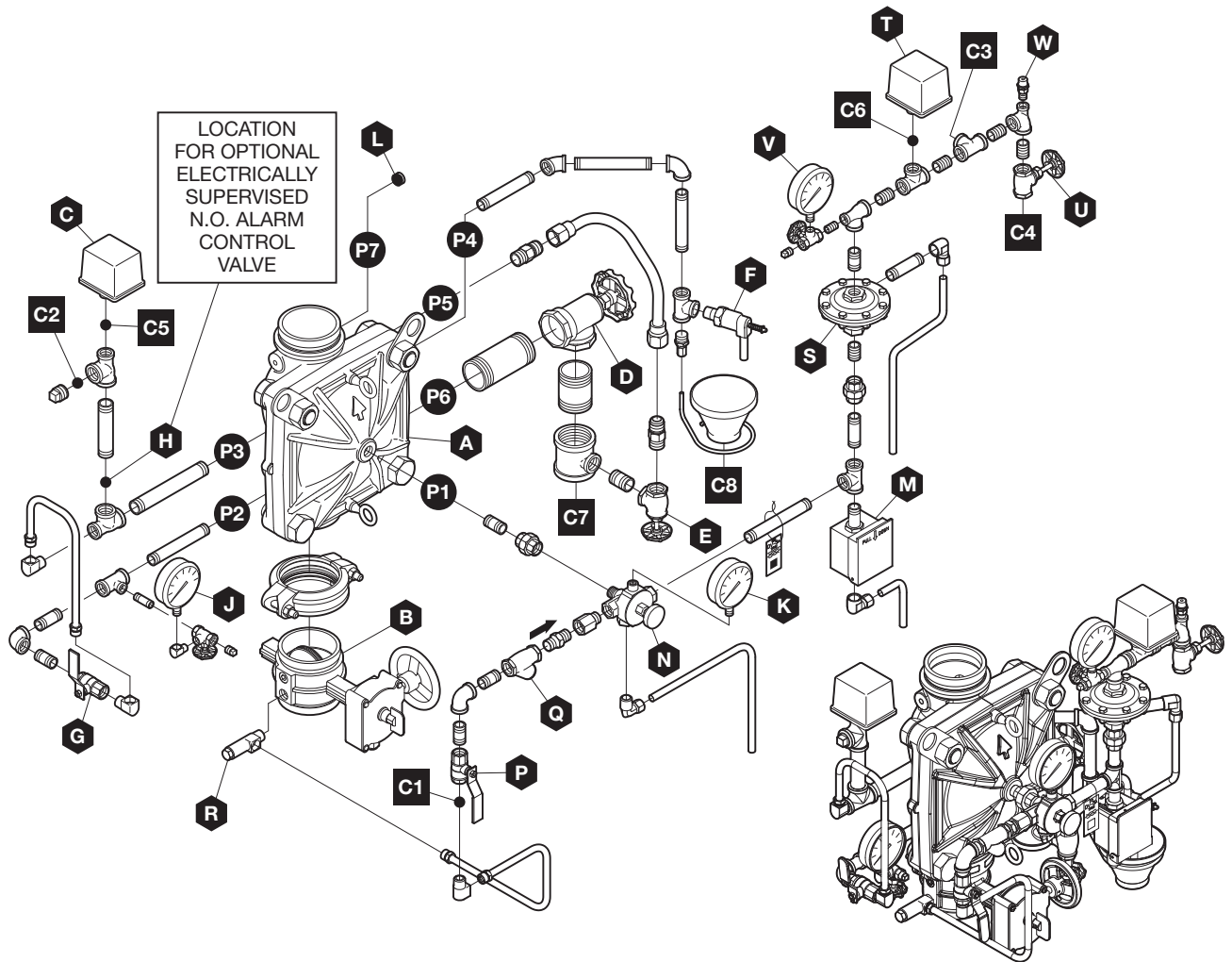
FIGURE 8 DV-5A VALVE DELUGE DRY PILOT ACTUATION TRIM (Refer To Figure 11 For Specific Bills Of Materials)
