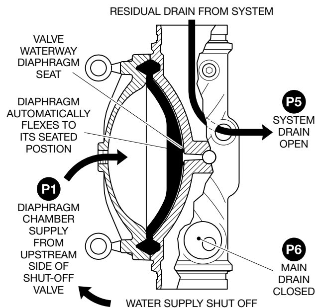
FIGURE 2 DV-5a VALVE OPERATION, DELUGE SYSTEMS
