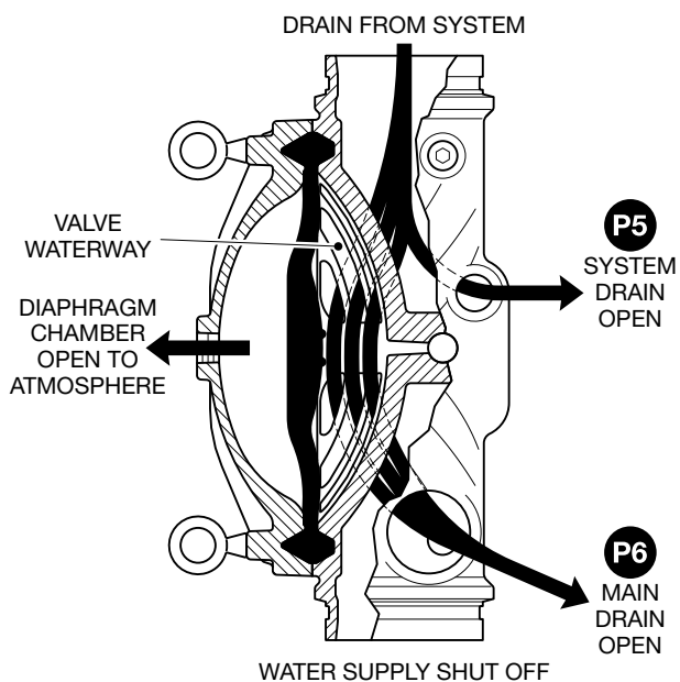
FIGURE 2 DV-5a VALVE OPERATION, DELUGE SYSTEMS
