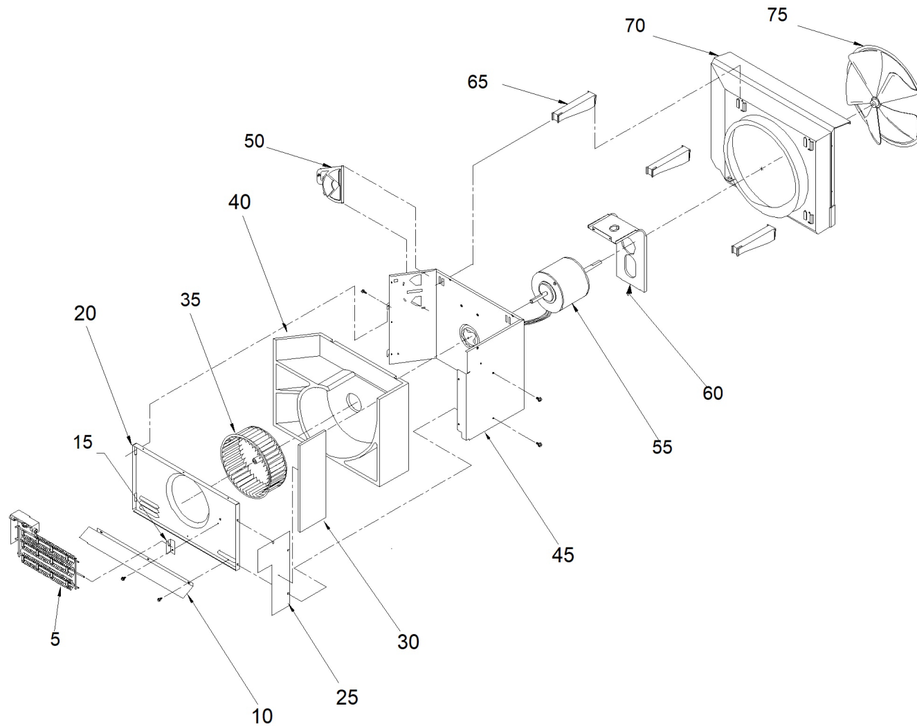
Figure 904 (Blower Module)
