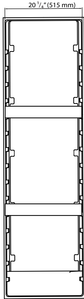
Front View
