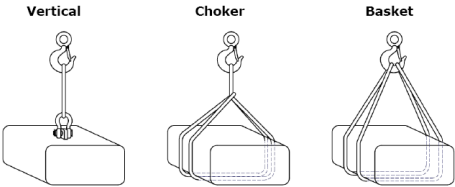
Figure 4-1. Common types of sling hitches
