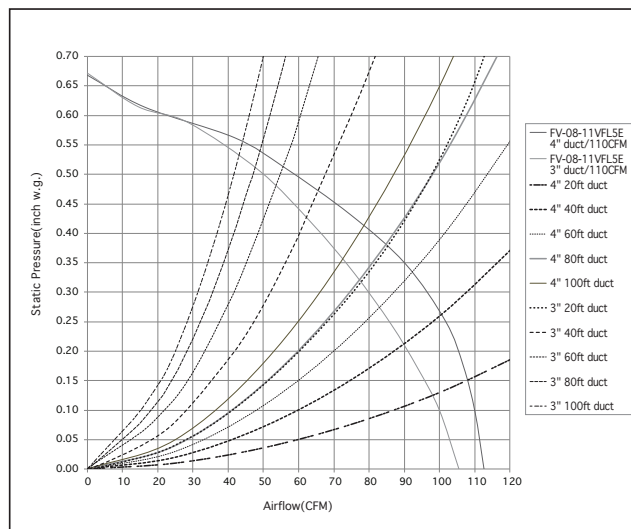
Performance Curve FV-08-11VFL5E - 110 CFM
