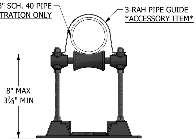
END VIEW
