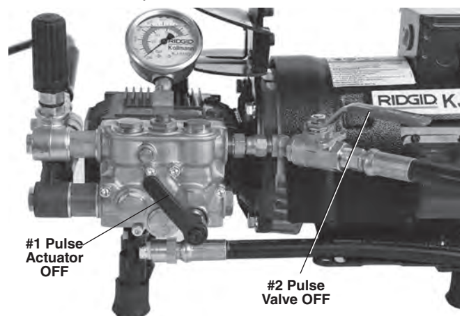
Figure 5 – Pulse Actuator/Pulse Valve OFF
