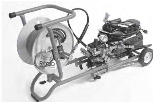
Figure 2B – Water Jetter with H-10 Cart and Hose Reel
