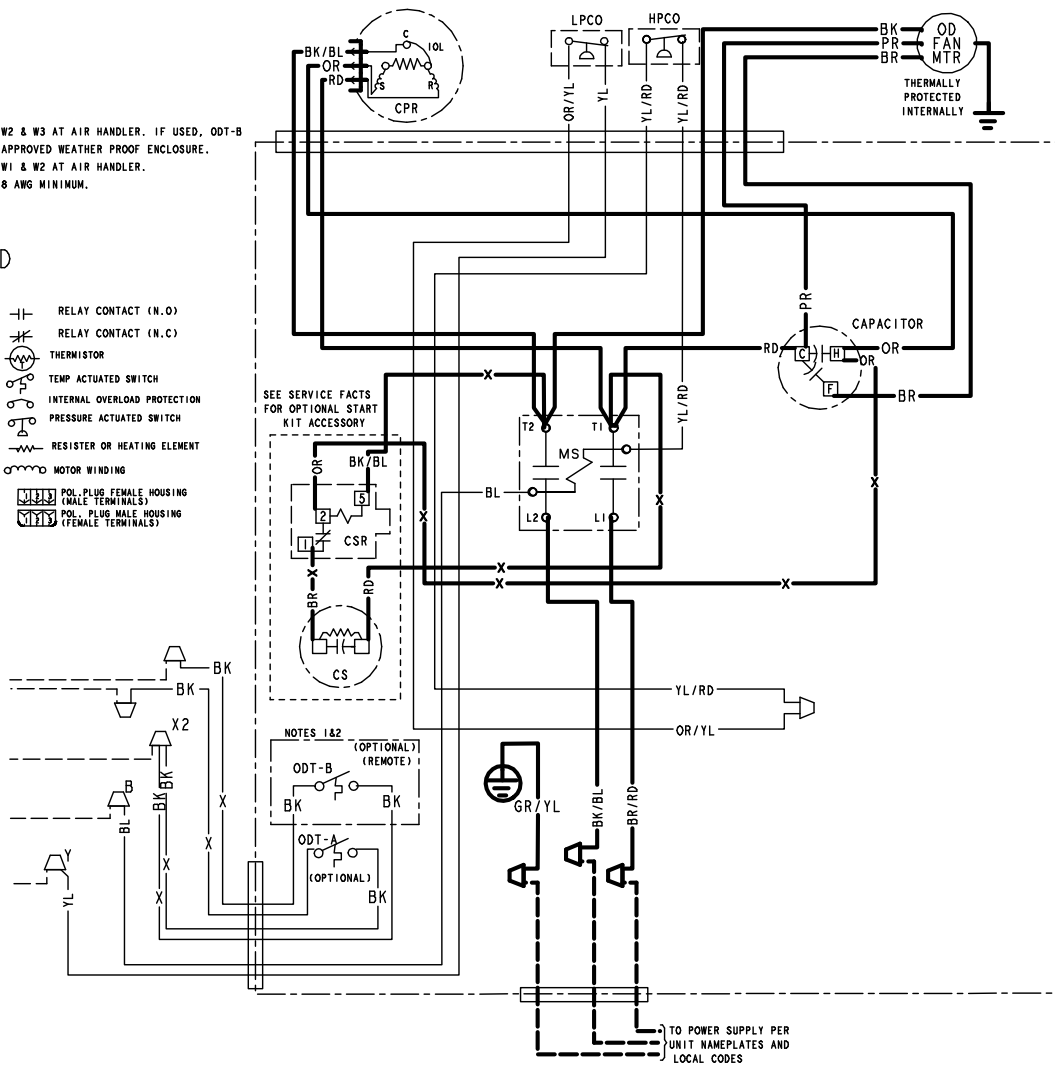
Figure 3. 5.0 Ton Models
