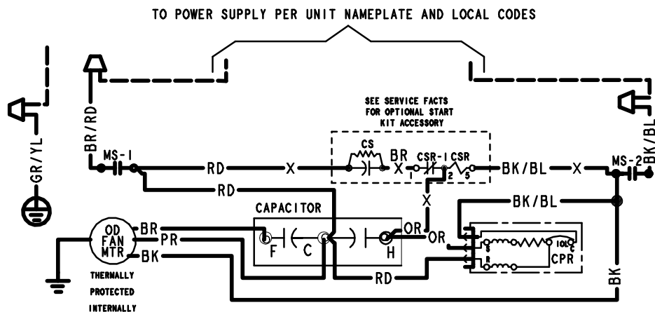
Figure 2. 5.0 Ton Models
