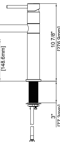
With Flange
