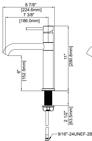
With Escutcheon
