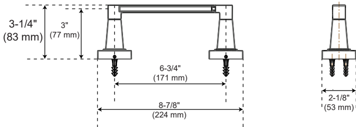
Pivoting Tissue Holder
