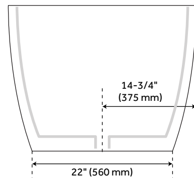
7" RIM HOLES
