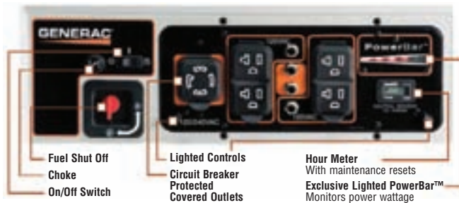
Convenient all-in-one Control Panel
