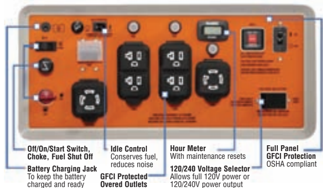
Easy Access all-in-one Control Panel
