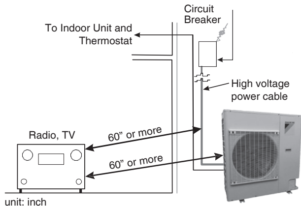
Placement to Minimize Electronic Noise
