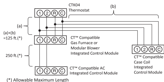
System Wiring (In case of CTK04)
