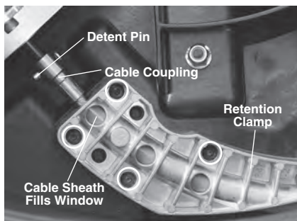
Figure 15 – Installing Cable Clamp
