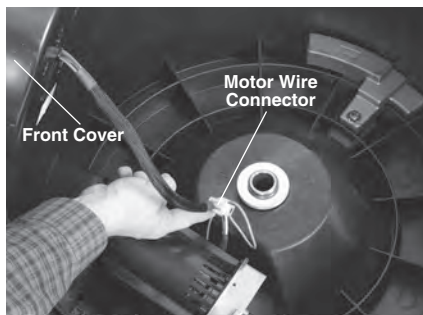
Figure 14 – Drain Cleaner Housing Opened
