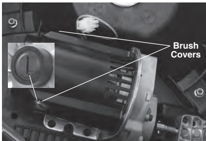
Figure 16 – Inspecting/Changing Motor Brushes
