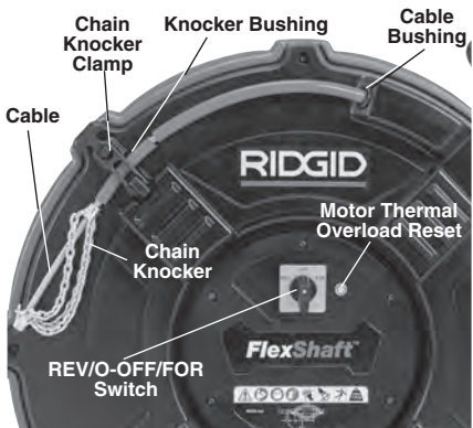
Figure 1C – Cable End/Chain Knocker
