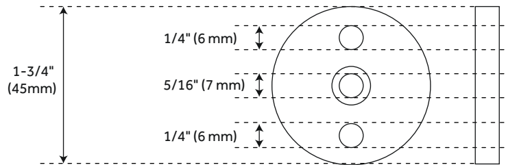
Round Rod Rail Mount Disk
