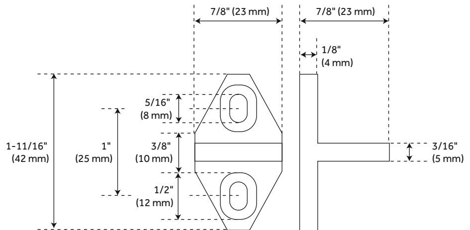
Mortise Floor Guide
