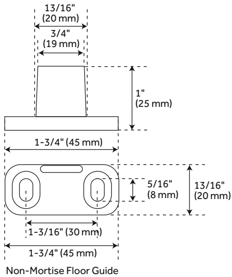
Non-Mortise Floor Guide
