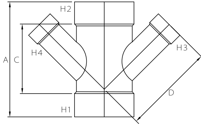
FABRICATED FITTING (F)
