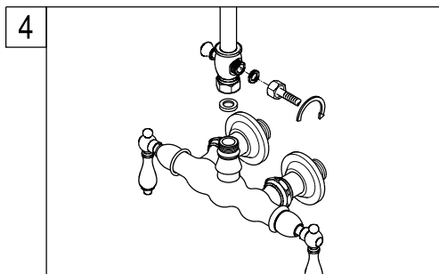
4. Install 60" add on shower kit to faucet body.
