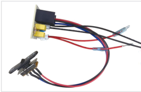
7. PCB-Switch Assy
