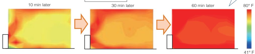
Air Distribution (MFZ-KJ15NA) (sectional view)
