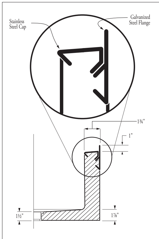
Construction Detail showing optional flange and cap.
