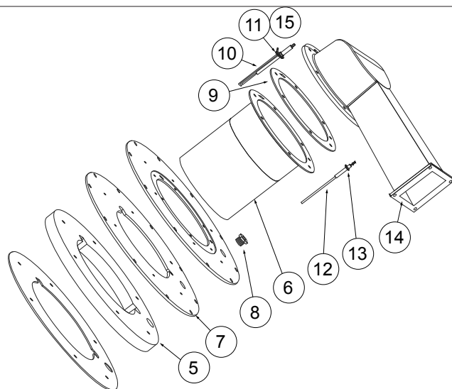
Burner Blower Assembly
