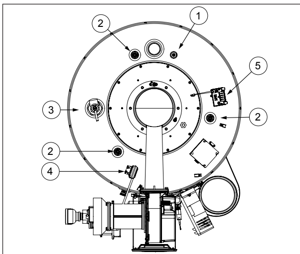
Top Components
