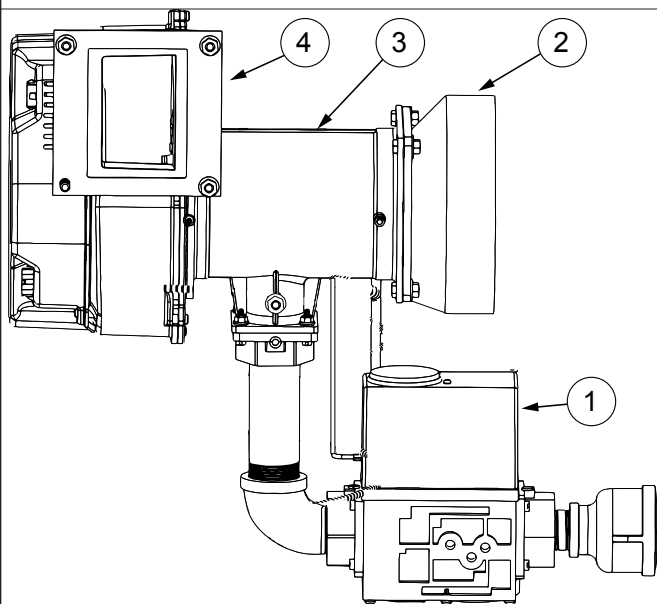
Gas Valve Assembly
