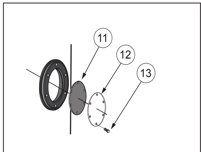
Cleanout Access
