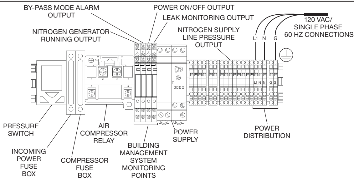
FIGURE 2B MODEL NG-1 100 AND NG-1 250 WALL-MOUNTED NITROGEN GENERATOR SYSTEM SIGNAL MONITOR AND 60 HZ POWER SUPPLY CONNECTION
