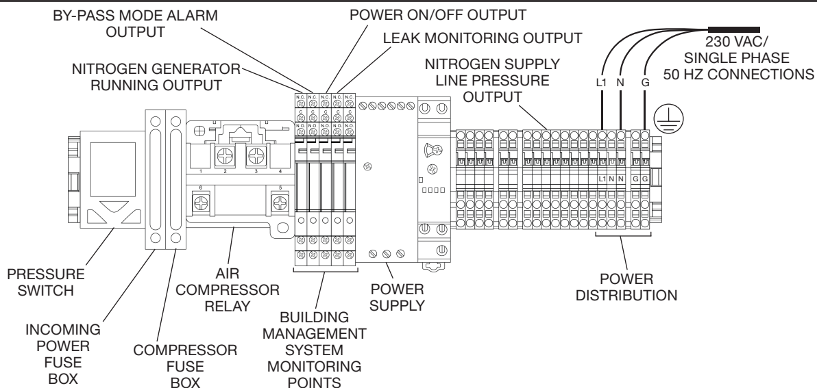
FIGURE 2A MODEL NG-1 100 AND NG-1 250 WALL-MOUNTED NITROGEN GENERATOR SYSTEM SIGNAL MONITOR AND 50 HZ POWER SUPPLY CONNECTION
