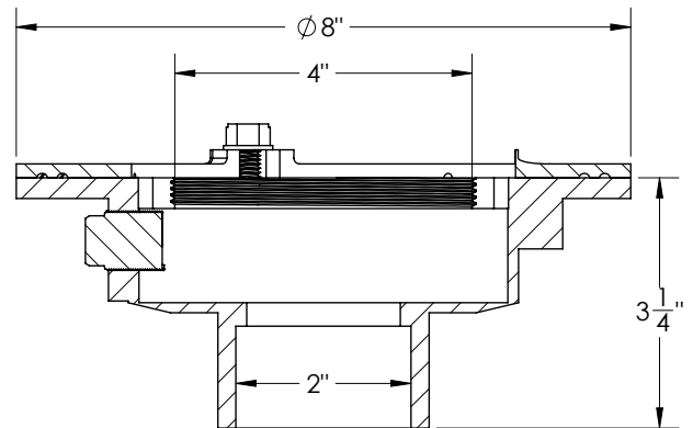
SECTION 1-1
