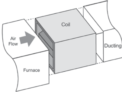
Fig 5B-2. Horizontal Right Application
