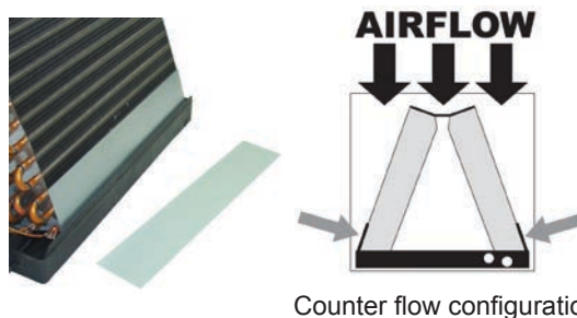
Fig 5A-3. Metal Plate location for a Downflow/Counterflow Application
