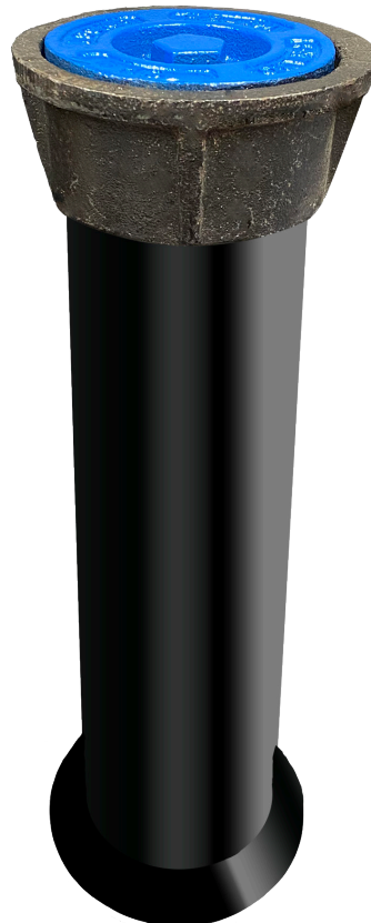
Part Number: TPITADJ-5T-*** TracerPit, All-Duty ADJ, 5-Terminal Lid (**Lid Color *Lid Message)
