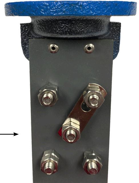
Part Number: TPITADJ-2T-*** TracerPit, All-Duty ADJ, 2-Terminal Lid (**Lid Color *Lid Message)
